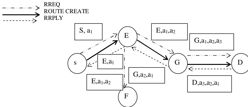
Figure 2: Secure based route creation
